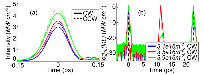
FIG. 8. 6.7mm ring cavity exhibits unstable unidirectionality at increasing pump powers. (a) The primary pulse output intensity profile highlights that unidirectionality exists between higher, and lower pump energy bidirectional setups. (b) The log plot of output intensity over one round trip demonstrates that unidirectionality is accompanied by the generation of a secondary pulse near one-half round trip.
