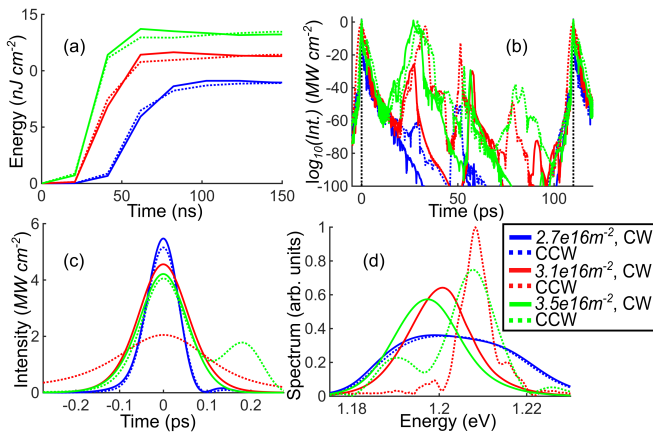
FIG. 7. Increasing pump energy through increasing carrier density comparison study for 33.5mm ring cavity. (a) The primary pulse energy grows more rapidly at increasing densities and converges to a higher value with only modest changes in relative intensities in counterpropagating pulses. (b) The final output intensity log plot over one round trip highlighting the generation of small secondary pulses. (c) The primary pulse output intensity and (d) spectra highlighting the destabilization and shifting spectral peaks at increasing carrier densities.
