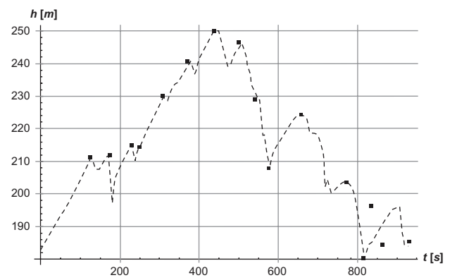
Figure 6 Simulated and experimental positions based on height h in meters as a function of time t in seconds along the track while skiing on snow using the skating technique. Notes: Dashed line: P = 253 Joules per second on uphill sections ( J/s ) and P = 197 J/s on downhill sections. ■: experimental values.
