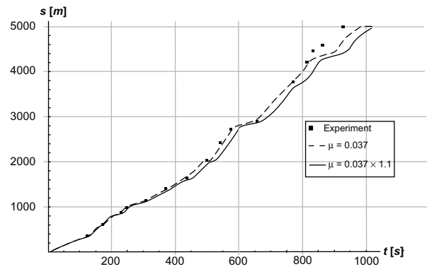
Figure 7 Simulated and experimental positions s in meters as a function of time t in seconds along the track while skiing on snow using the skating technique. Notes: P = 253 Joules per second ( J/s ) on uphill sections and P = 197 J/s on downhill sections. Dashed line: \mu = 0.037 ; Solid line: \mu = 0.037 \times 1.1 ; ■: Experimental values.
