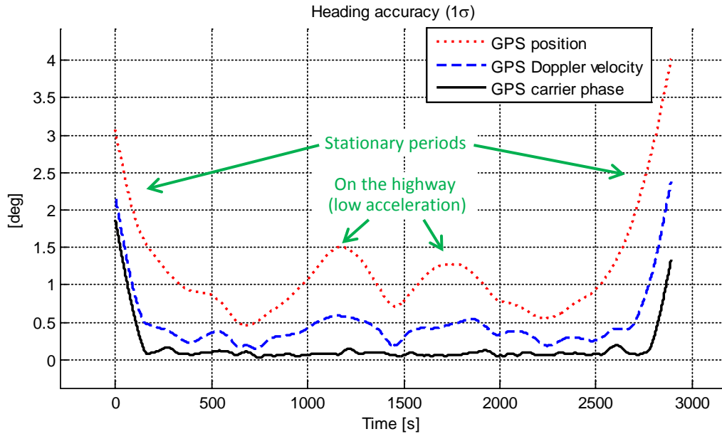
Figure 3. The heading accuracy from Method 7 in the car test varied with acceleration and with different methods to find \mathbf{a}_{EB}^E . The car had a stationary period before driving on smaller roads, and then a period on a highway, before driving back the same way. The three graphs show theoretical uncertainty in smoothed heading when NavLab is aided with GPS position ( \mathbf{p}_{EB}^E ) or GPS velocity ( \mathbf{v}_{EB}^E ) from Doppler shift or carrier phase. Only the uncertainty with GPS position aiding is verified with an external heading reference, the two others are simulated with accuracies based on u-blox (2015) and van Graas and Soloviev (2004).
