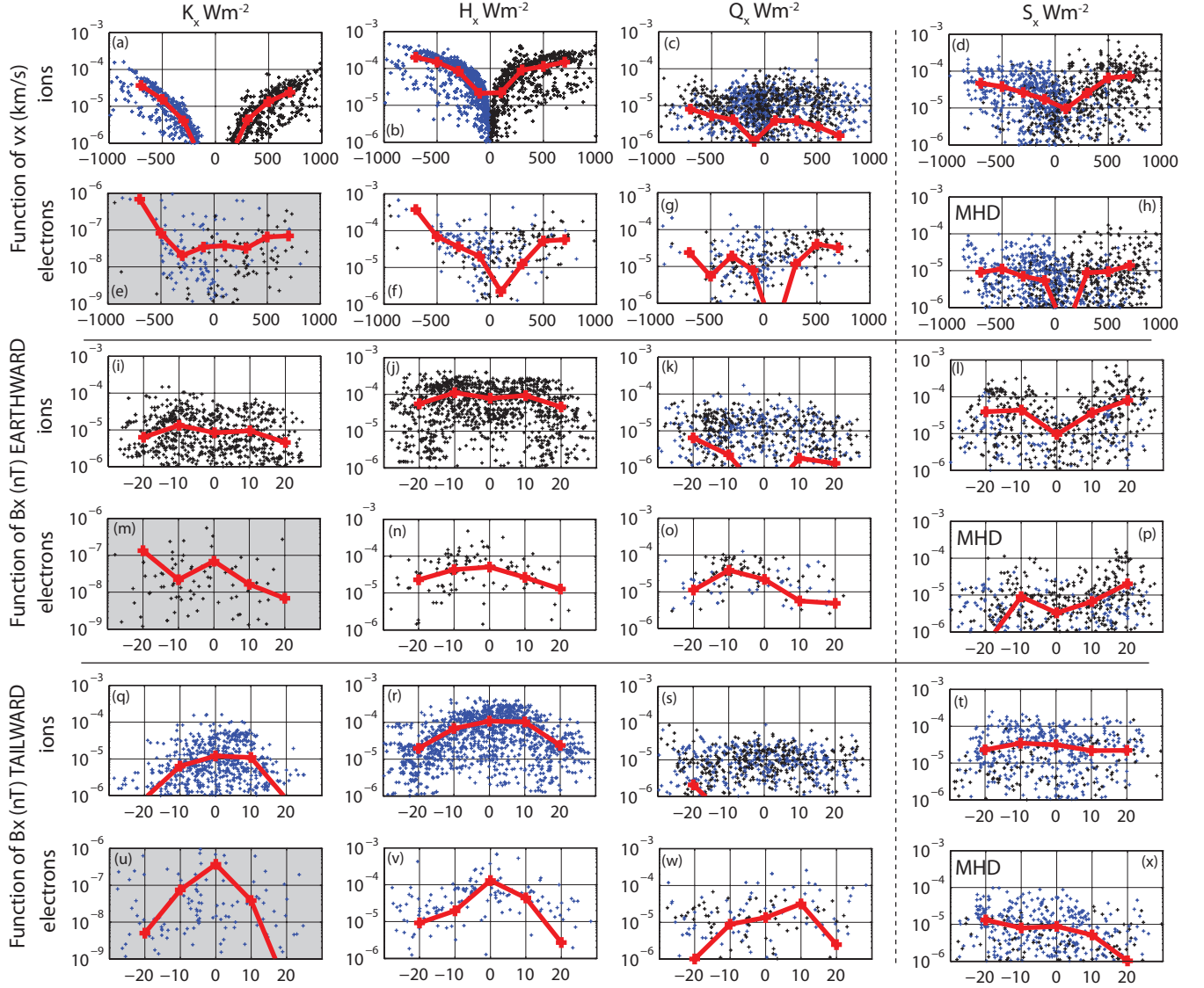
FIG. 2: (a-h) Energy fluxes as a function of outflow speed v_x , (i-p;q-x) as a function of the reconnecting component of the magnetic field B_x in the Earthward and tailward directions.
