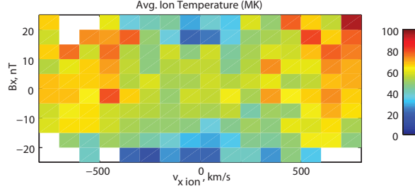
FIG. 3: Ion temperature as a function of outflow speed v_x and reconnecting component of the magnetic field B_x .
