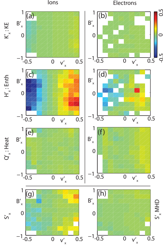
FIG. 5: Average normalised energy flux as a function of both v_x and B_x . Cells with no data are colored white
