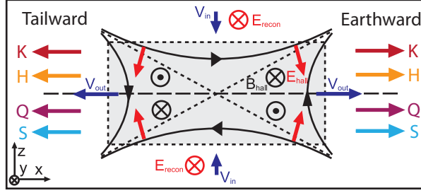
FIG. 1: The geometry of the reconnection X-line in the Earth's magnetotail.
