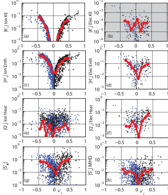
FIG. 4: Normalized absolute energy fluxes as a function of v_{i,x}/v_A .
